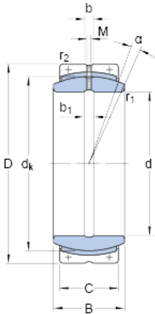
GEC 360 FBAS Bearing 2D drawings and 3D CAD models
